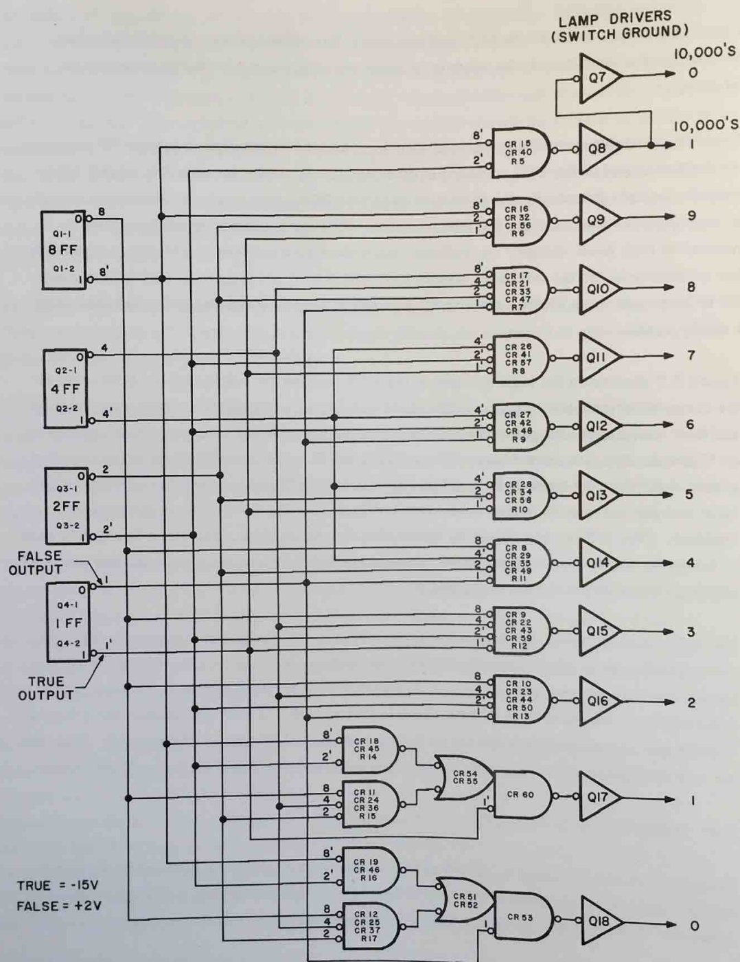
Figure 3.7. Decoding Matrix and Light Drivers, Logic Diagram
