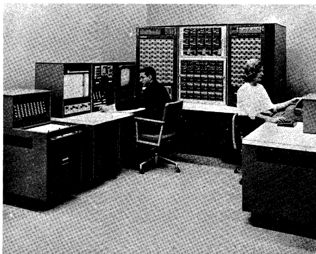
Figure 19—8800 100V transistorized computer with display wing
