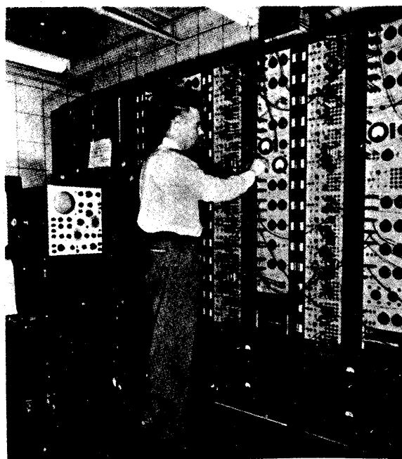
Figure 5—Boeing analog computer, courtesy of Boeing Airplane Co.
