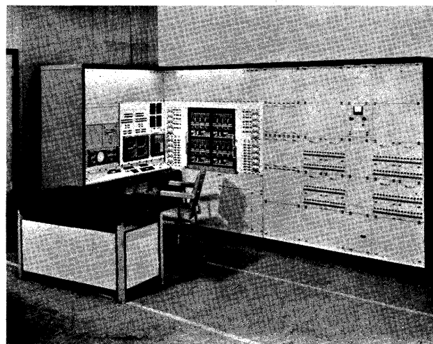
Figure 15—Applied Dynamics large scale 256 amplifier computer
