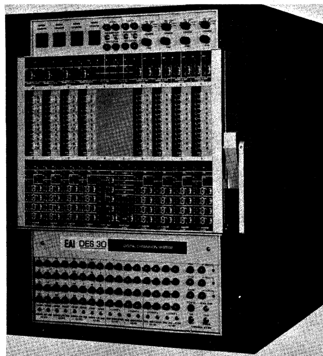
Figure 14—Digital expansion system by EAI (allows parallel patchable digital logic expansion to 10 volt systems, in a self-contained desk top frame)
