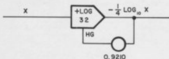
Figure A4.11. Base 10 Log
