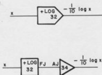
Figure A1.32. Logarithm, Using the +Log Network
