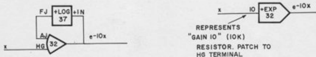
Figure A1.34. Exponential, Using the +Network
