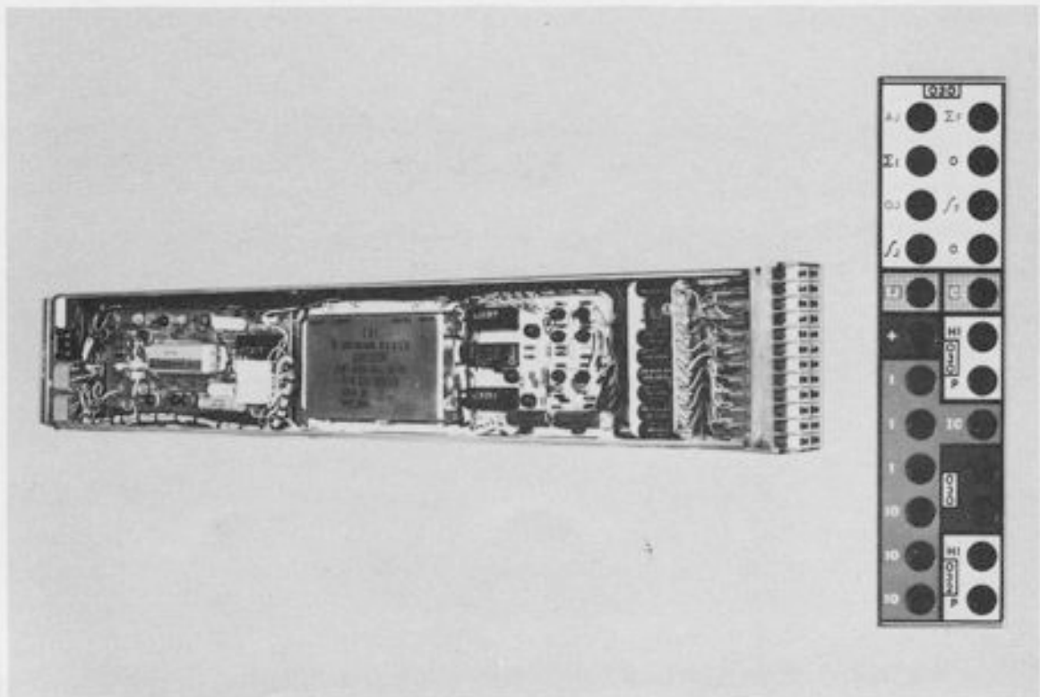
Figure 5.1. A Typical Tray and its Patching Area
