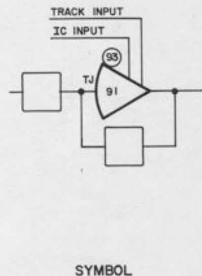
Figure A1.14. Track/Store Unit with Arbitrary Feedback
