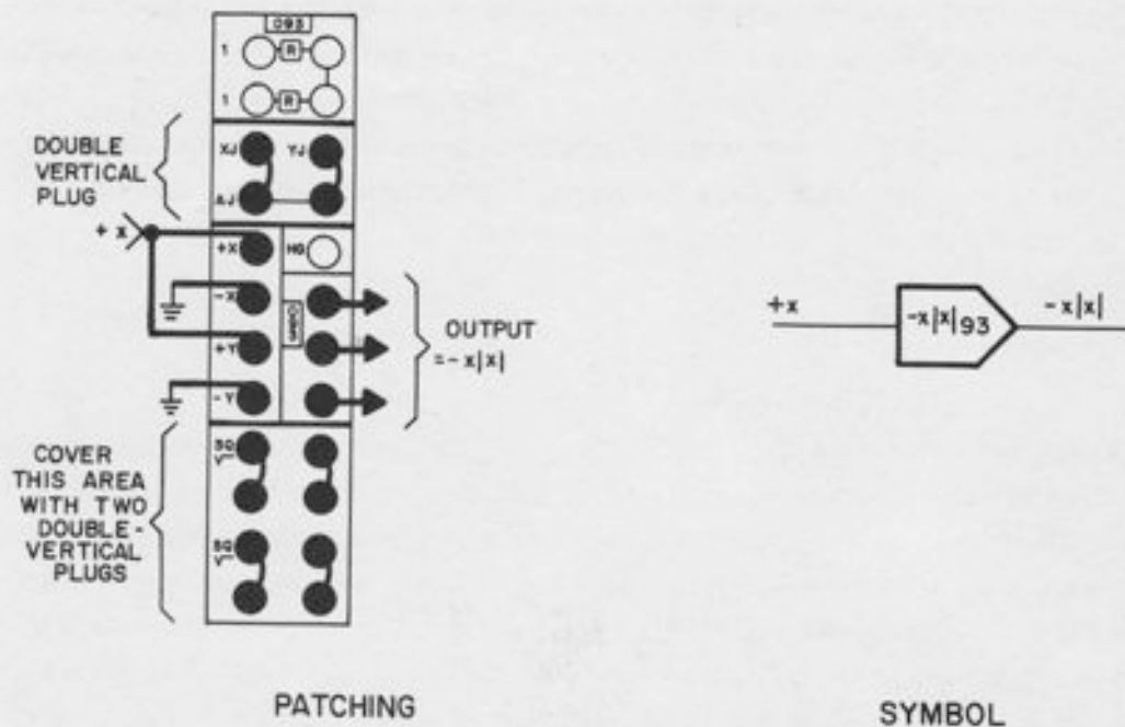
Figure A1.30. Generating -x|x|
