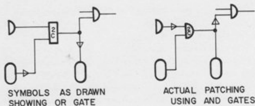
Figure 14.2. Using an AND Gate for the OR Function
