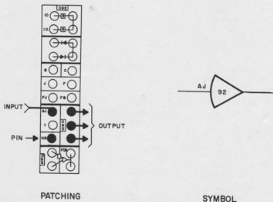
Figure A1.16. Using the Junction Inverter as a High-Gain Amplifier
