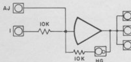
Figure 9.1. Simplified Schematic, Junction Inverter
