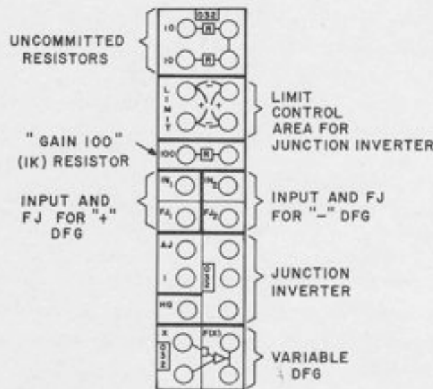
Figure 9.5. The Log/Exponential DFG Patching Terminations
