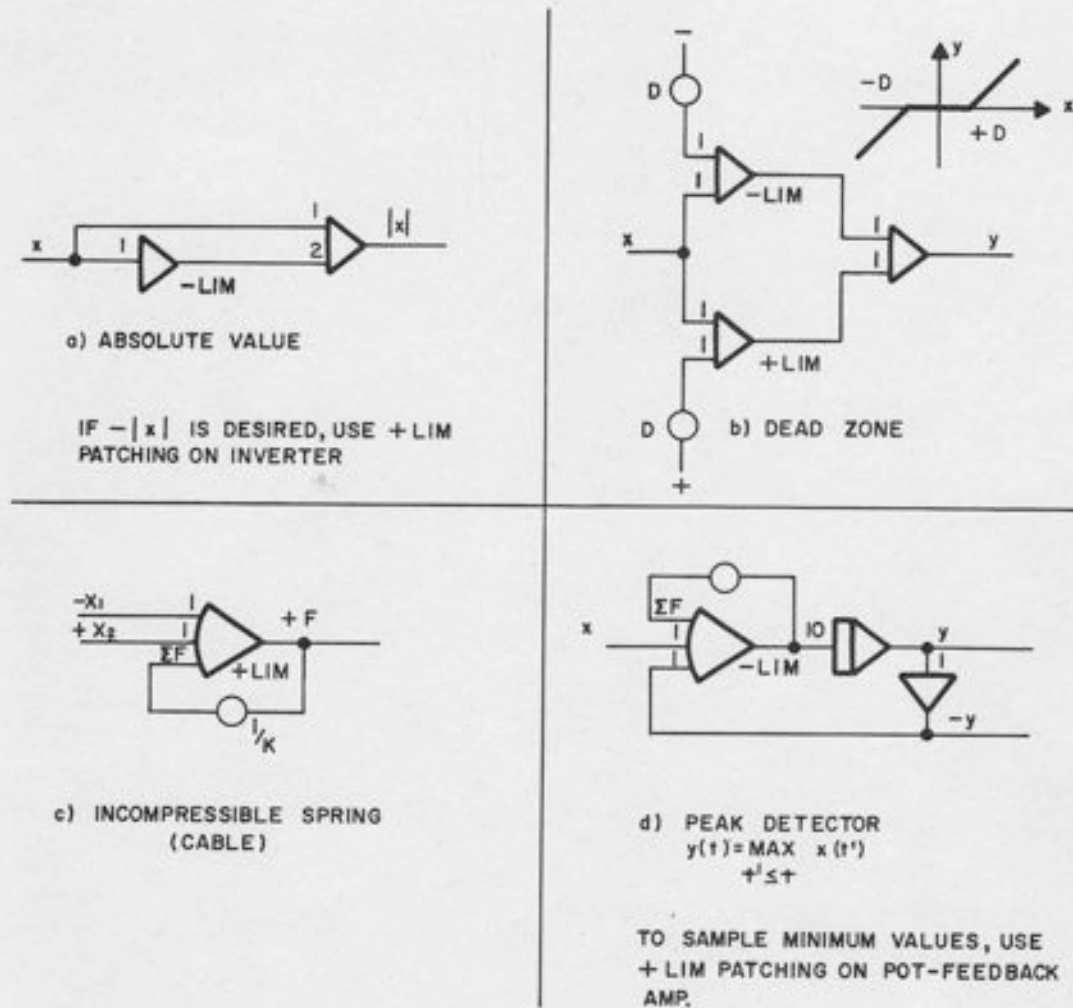
Figure 7.4. Typical Applications of the Limit Summer
