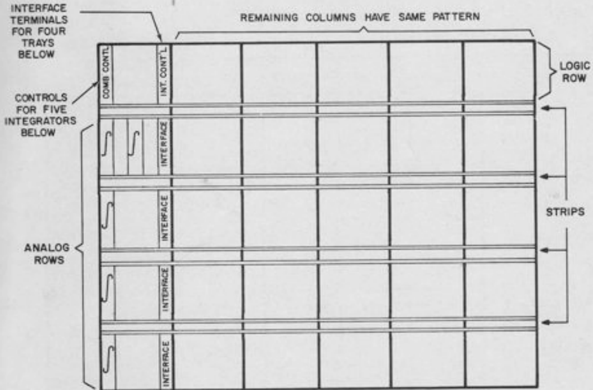
Figure 5.2. Patch Panel Layout, Showing Rows, Strips, and Fields
