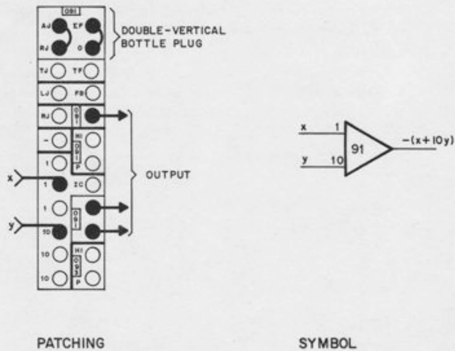
Figure A1.6. Summation with a Track/Store Summer
