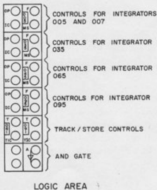
Figure 6.1. Patch Panel Layout for Combination Amplifier
