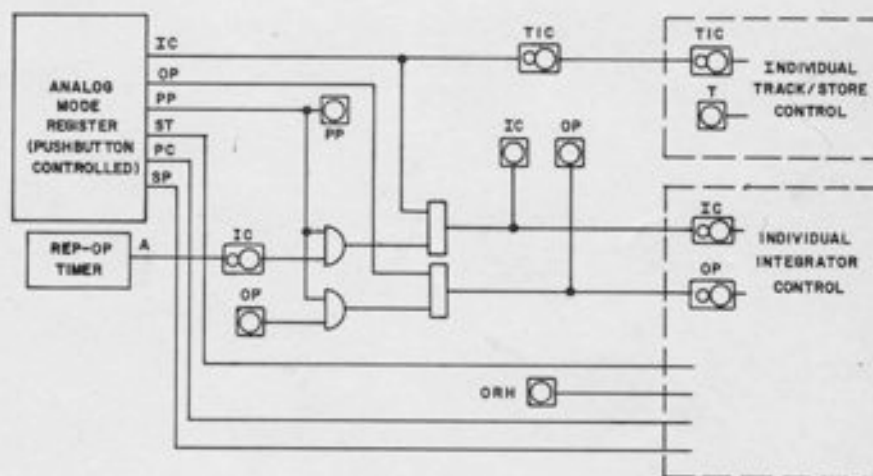
Figure 20.3. Mode Register and Mode Control Logic
