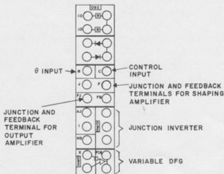
Figure 9.6. Patching Terminations for Sin/Cos DFG
