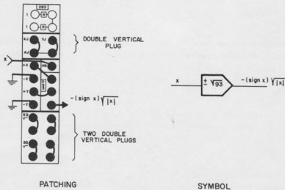
Figure A1.31. Generating -(\text{sign } x)\sqrt{|x|}
