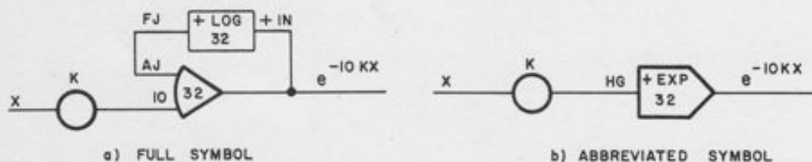
Figure A4.1. Basic Exponential Circuit
