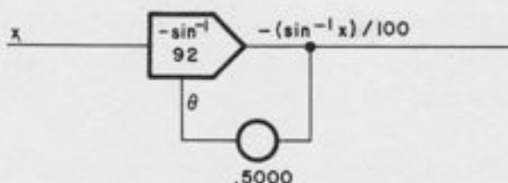
Figure A1.38. Inverse Sine Function with Pot Feedback
