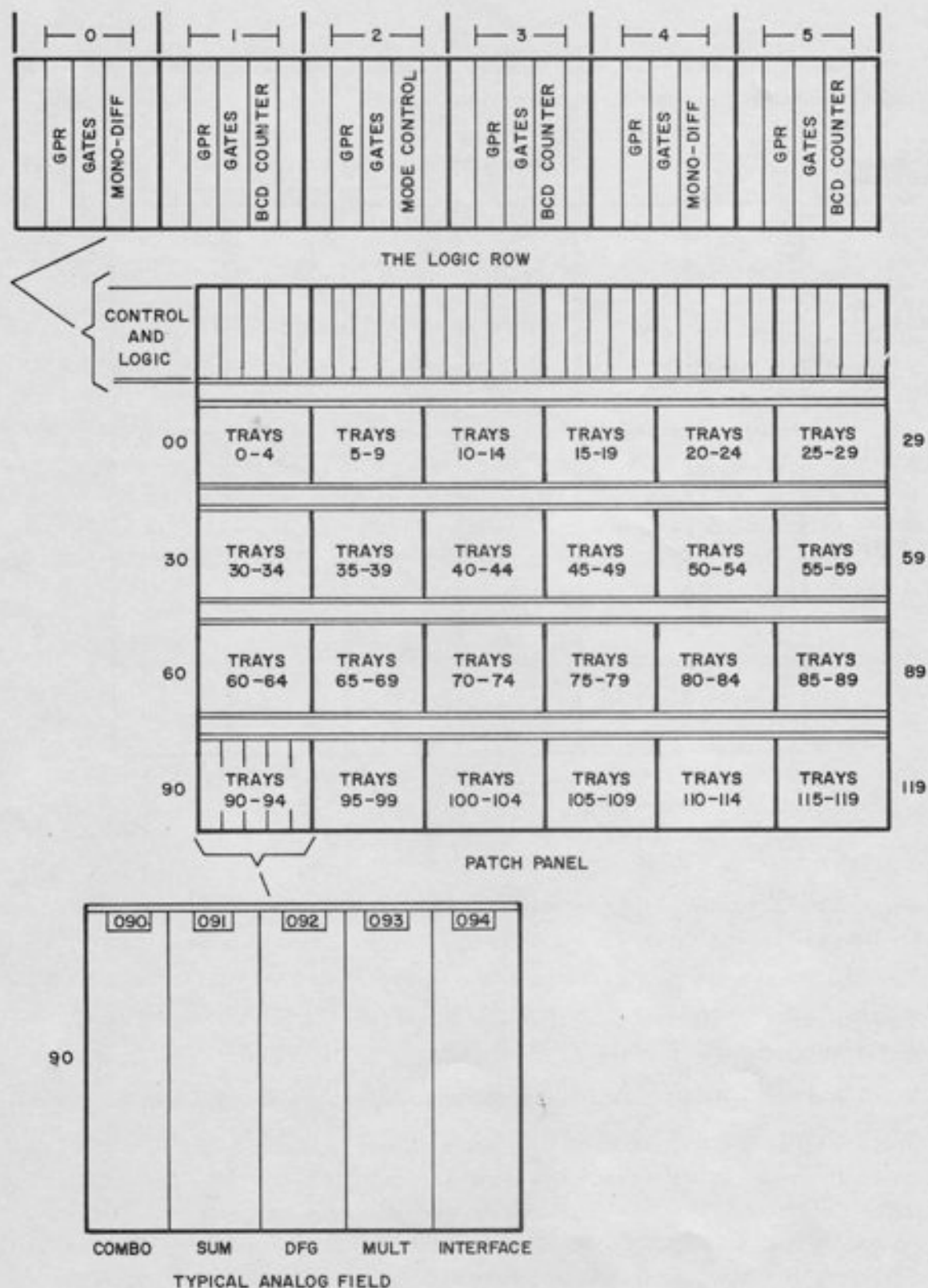
Figure 5.3. Detailed Patch Panel Layout
