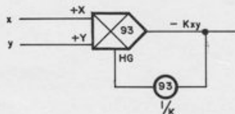
Figure A1.25. Multiplication with Pot Feedback
