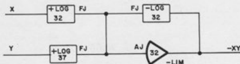
Figure A4.5. Multiplication - Single Amplifier
