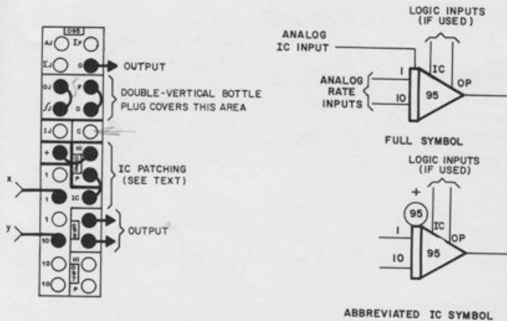
Figure A1.2. Standard Patching and Symbols for an Integrator
