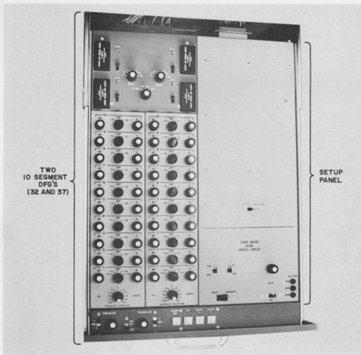
Figure 10.4. DFG Setup Panel (In Upper DFG Drawer)
