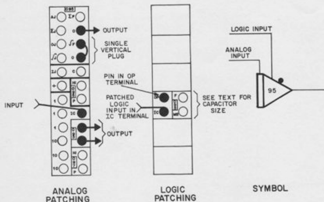
Figure A1.15. Using the Combination Amplifier as a Track/Store Unit
