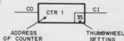
Figure 16.2. Programmer's Symbol for BCD Counter
