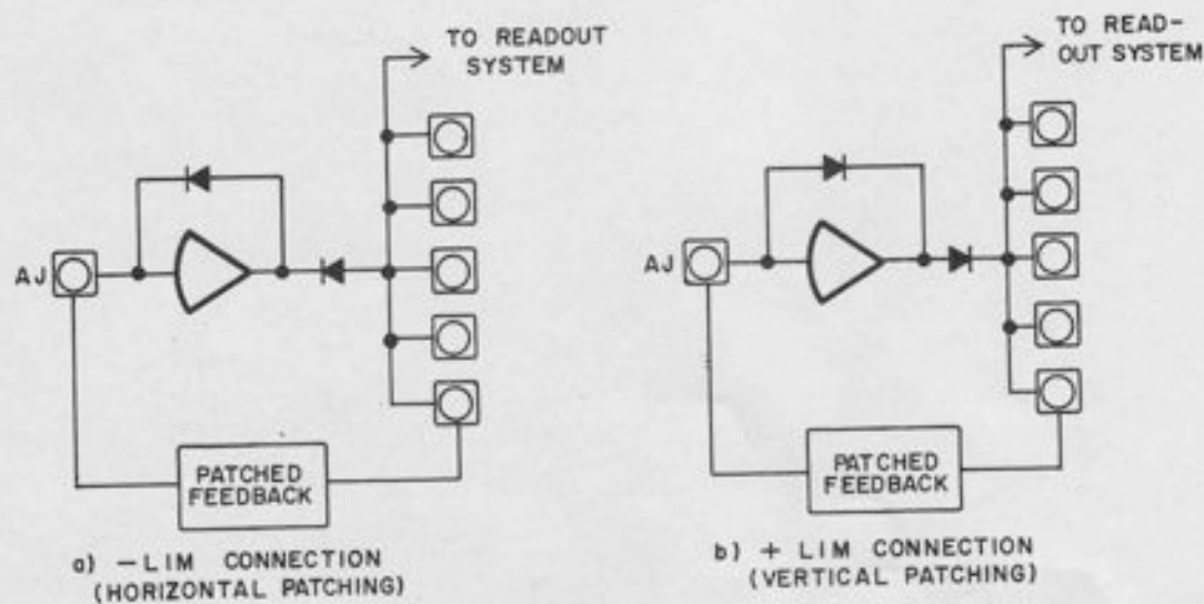
Figure 7.6. Equivalent Circuits of Limit Summer with Bottleplug Inserted
