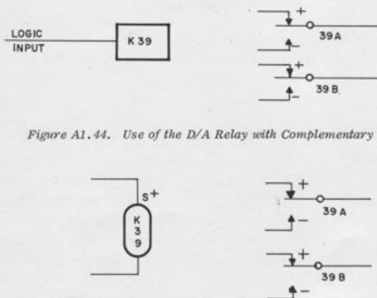
Figure A1.45. Use of the D/A Relay as a Latching Relay
