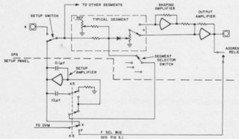
Figure 10.11. Setup Panel Circuitry
