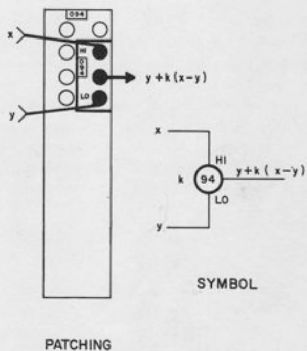
Figure A1.23. Three-Terminal Pot, Typical Symbol and Patching
