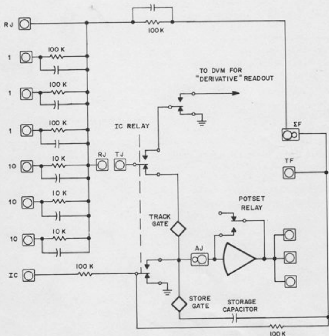
Figure 7.2. Simplified Schematic of Track/Store Summer
