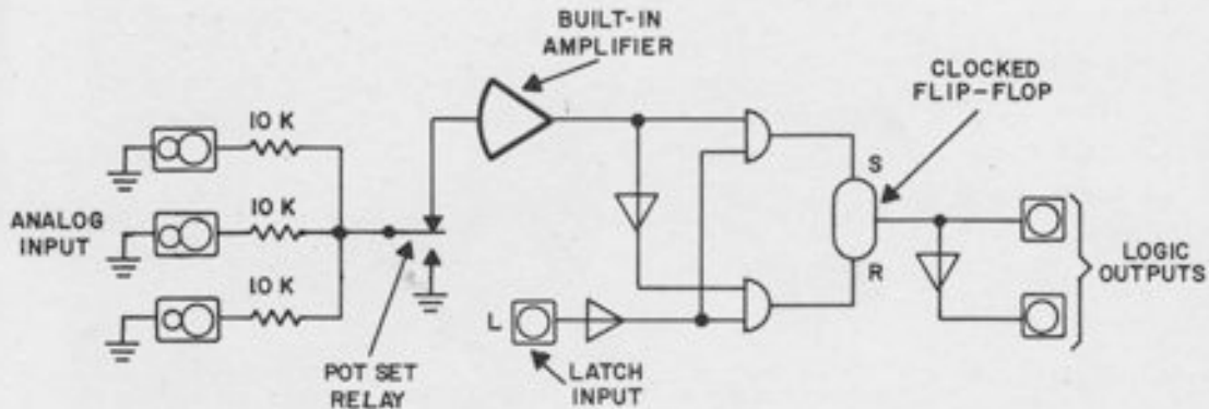
Figure 13.2. Block Diagram, Electronic Comparator
