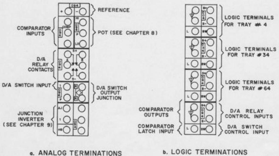
Figure 13.1. Interface Tray Terminations
