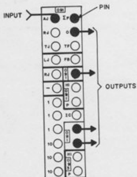
Figure A1.17. Using the Limit Summer as a High-Gain Amplifier
