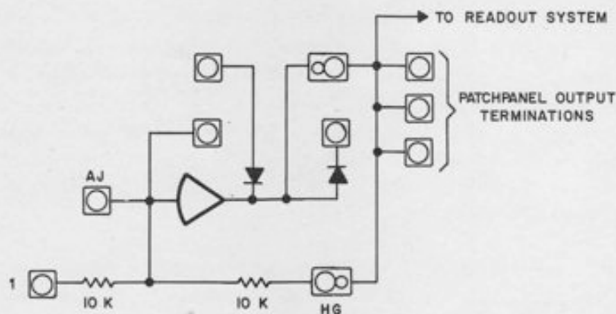
Figure 9.4. Simplified Schematic, Junction Inverter with Zero Limiting
