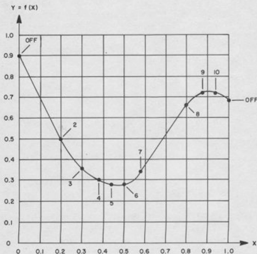
Figure 10.2. Typical Ten-Segment Function
