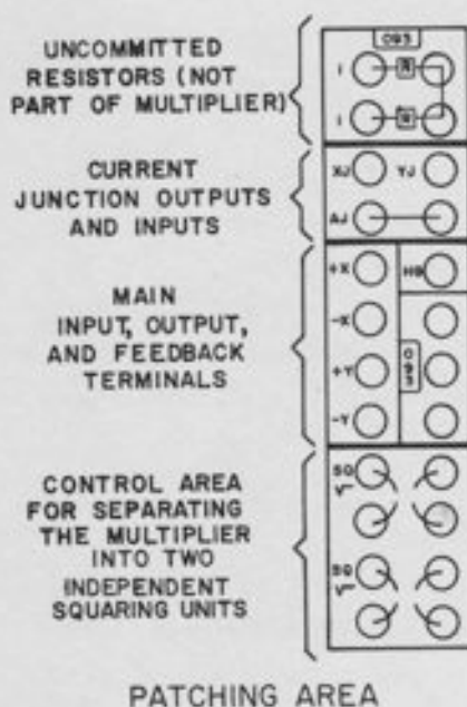
Figure 11.1. Quarter-Square Multiplier Patching Area
