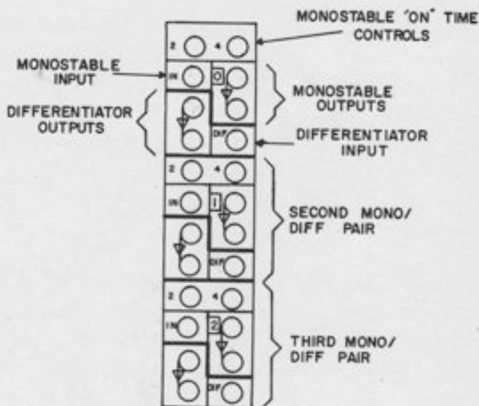
Figure 17.1. Patch Panel Terminations for Mono/Diff Tray
