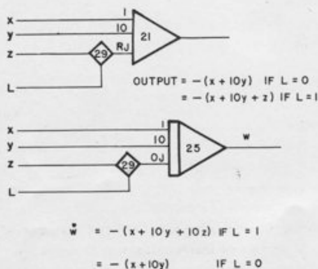
Figure A1.42. Programmer's Symbol for D/A Switch
