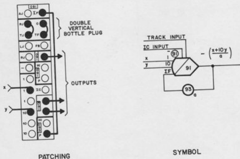
Figure A1.13. Track/Store Unit with Pot Feedback
