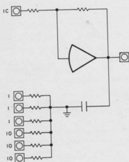
Effective circuit for integrator in IC mode. (Hold circuit eliminated for clarity. Note that the feedback capacitor and the input resistor are grounded.)
