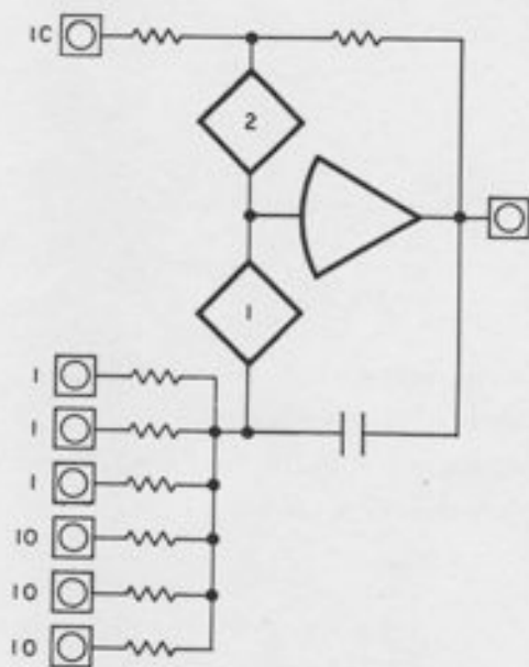
Simplified schematic for integrator. (HOLD mode circuitry omitted for clarity.)
