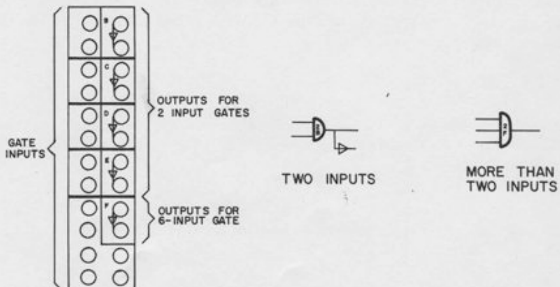
Figure 14.1. Patch Panel Terminations and Programmer's Symbols for AND Gates
