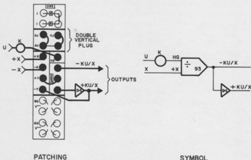
Figure A1.26. Symbol and Patching for Division
