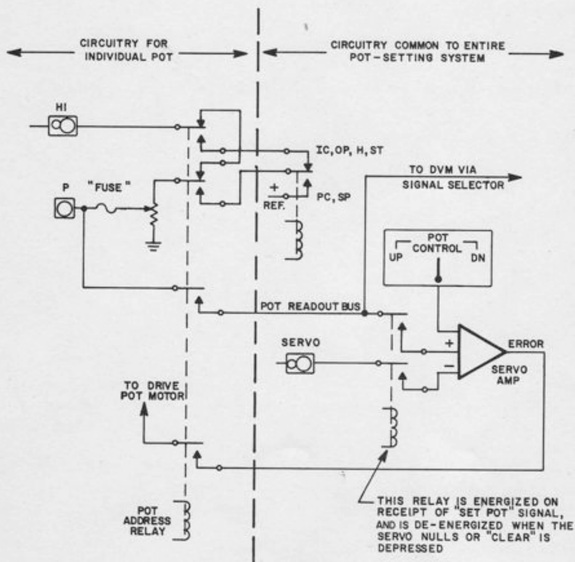
Figure 4.2. Individual Pot Addressing Circuitry
