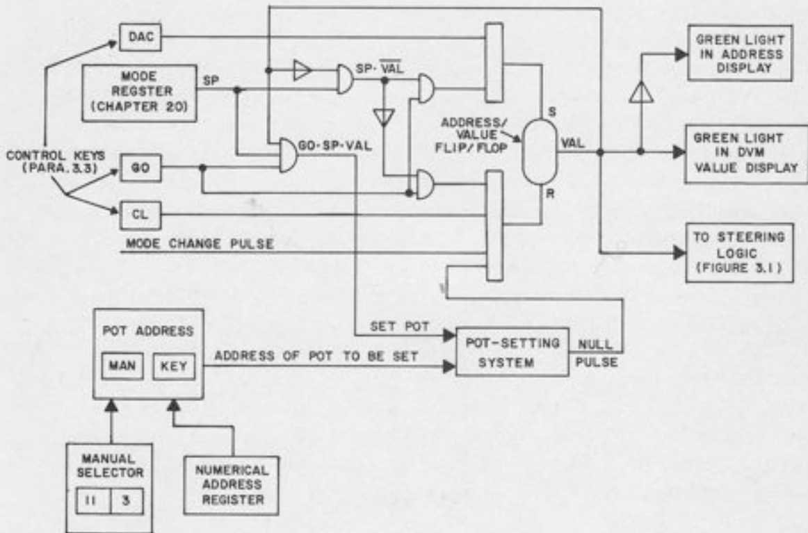
Figure 4.1. Logic Diagram of Servo Pot-Setting System
