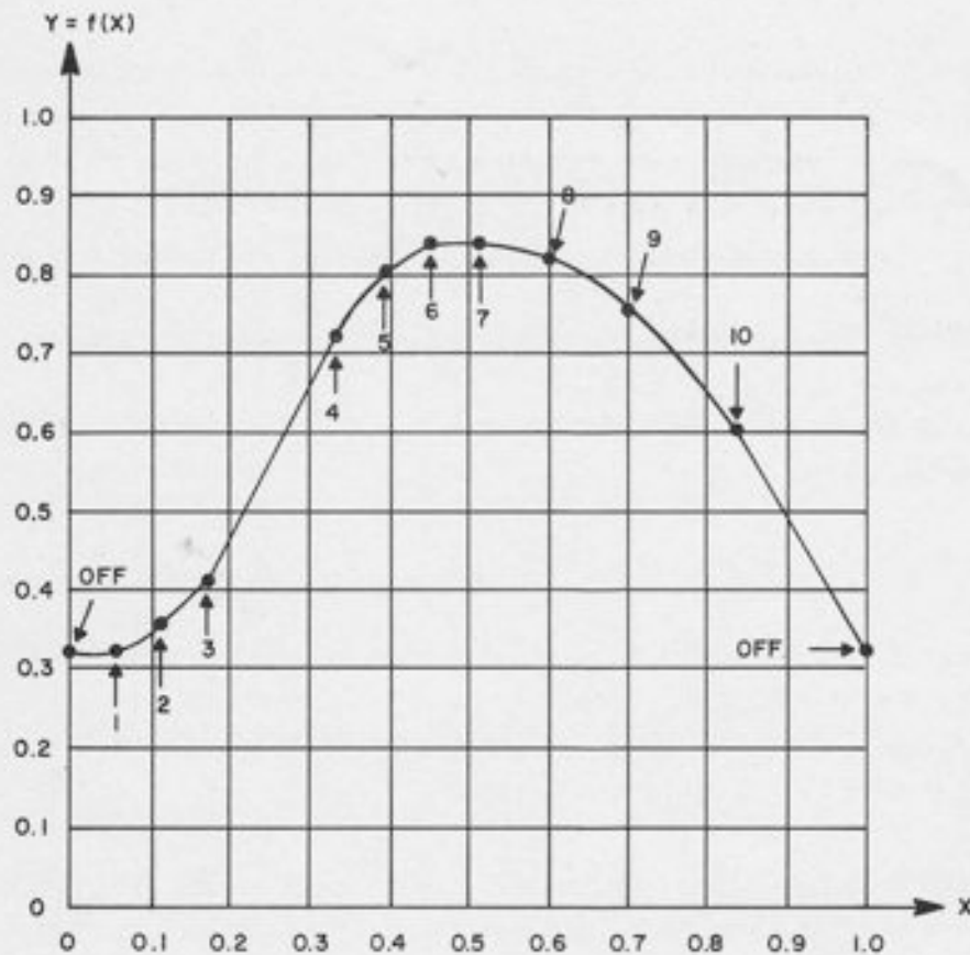
Figure 10.7. Initially Horizontal Eleven-Segment Function
