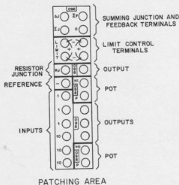
Figure 7.3. Patching Area for Limit Summer
