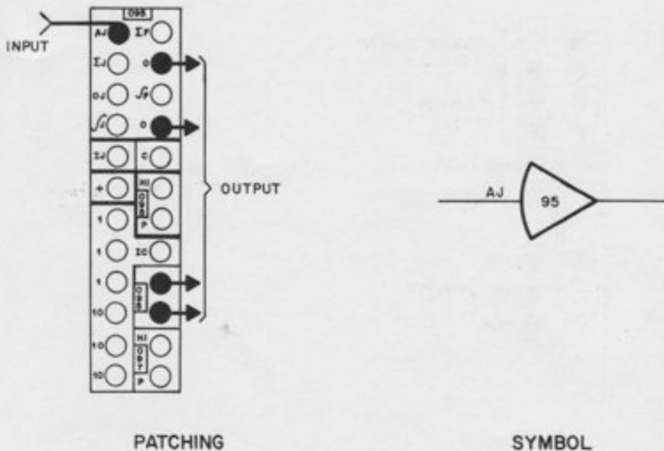
Figure A1.19. Using the Combination Amplifier as a High-Gain Amplifier
