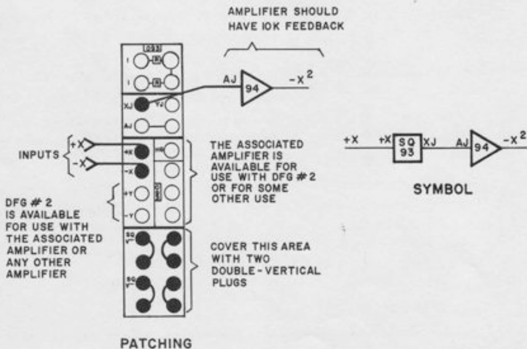
Figure A1.28. Squaring with DFG 1 and Another Amplifier
