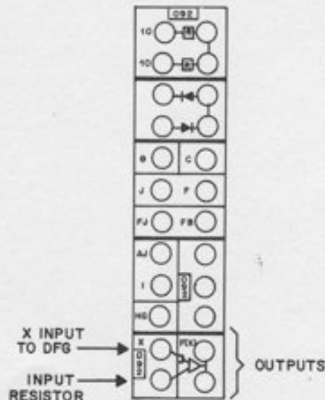
Figure 10.1. Variable DFG Patching Terminations
