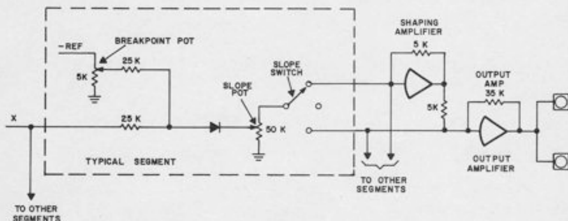
Figure 10.9. Typical Circuitry for One Segment
