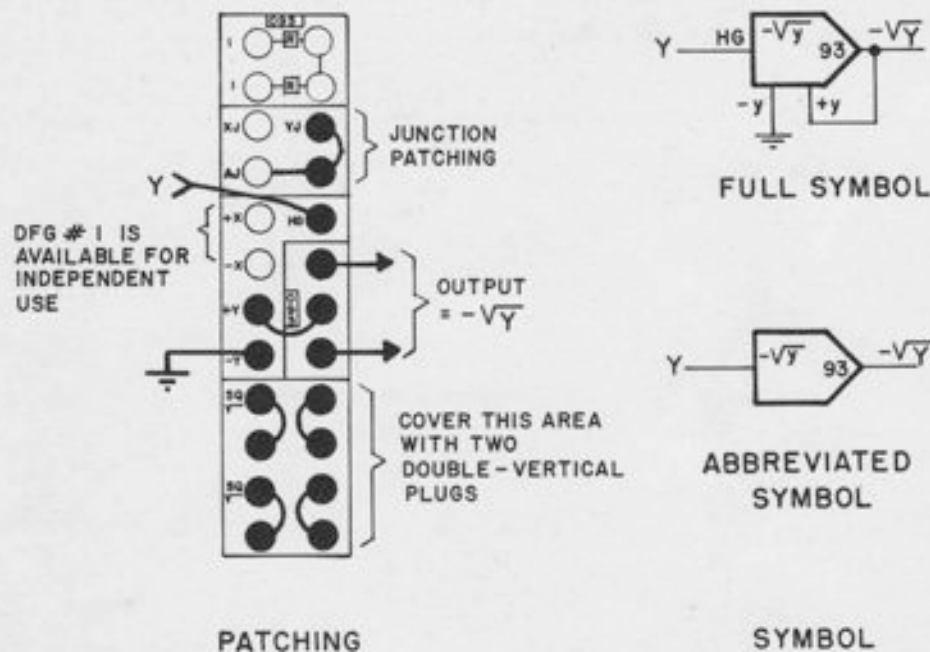
Figure A1.29. Square Root Circuit, DFG 2
