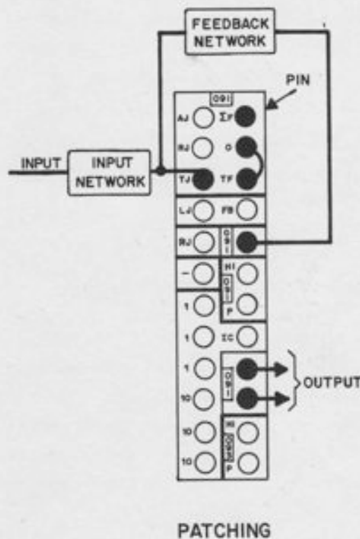
Figure A1.14. Track/Store Unit with Arbitrary Feedback
