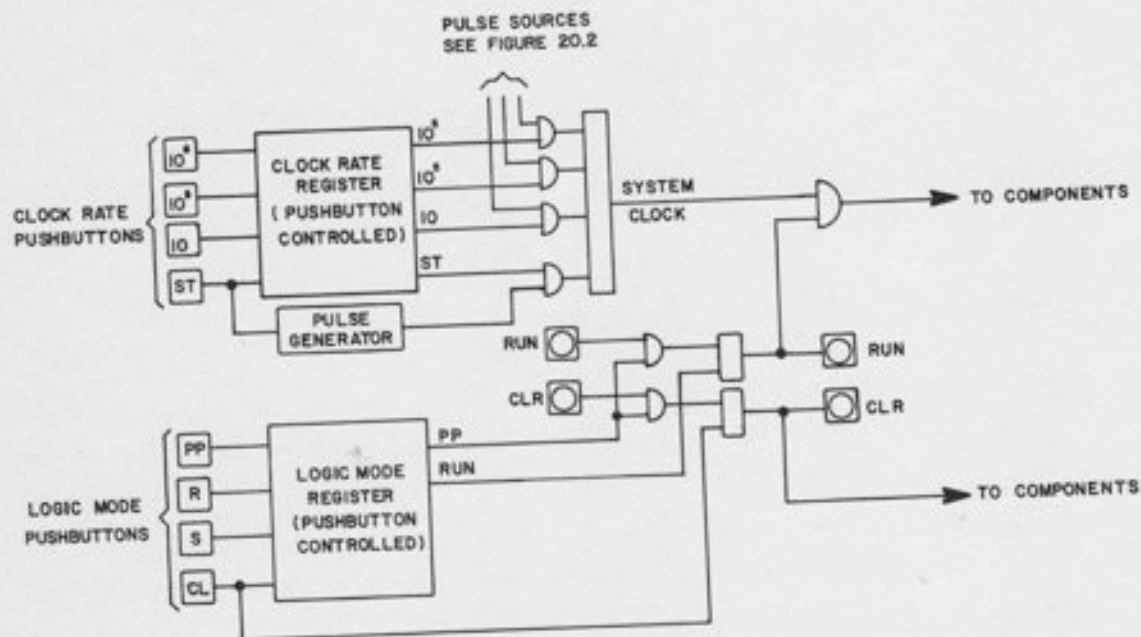
Figure 21.1. Logic Diagram of the Logic Mode and Clock Rate Control
