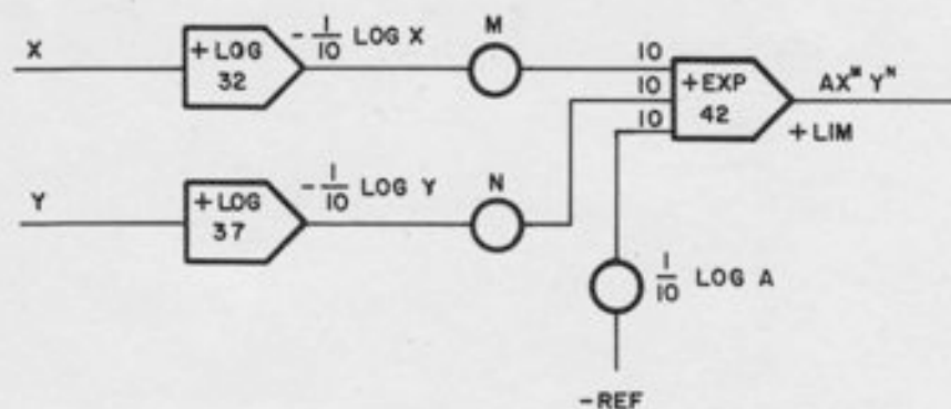
Figure A4.8. Products of Powers
