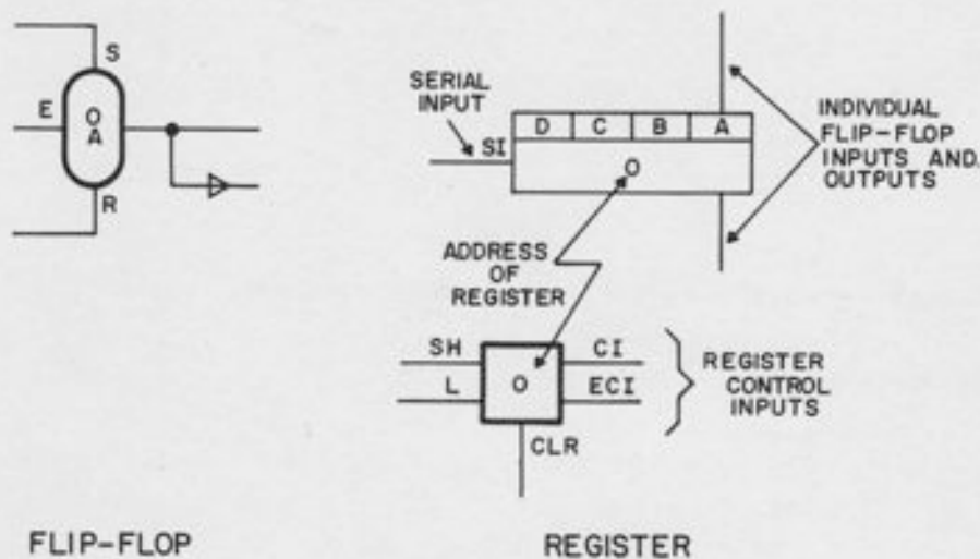
Figure 15.3. Programmer's Symbol for a Flip-Flop and a Register
