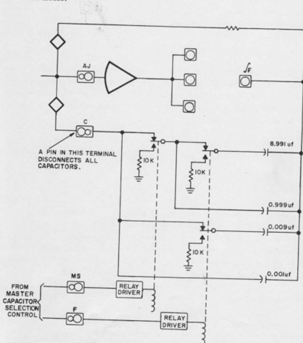
Figure 6.3. Simplified Schematic of Capacitor Selection Circuitry
