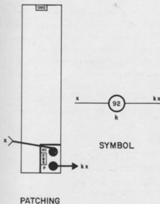
Figure A1.22. Two-Terminal Pot, Typical Symbol and Patching
