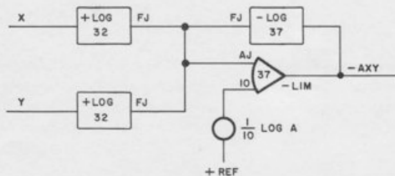
Figure A4.7. Multiplication with Arbitrary Scale Factor
