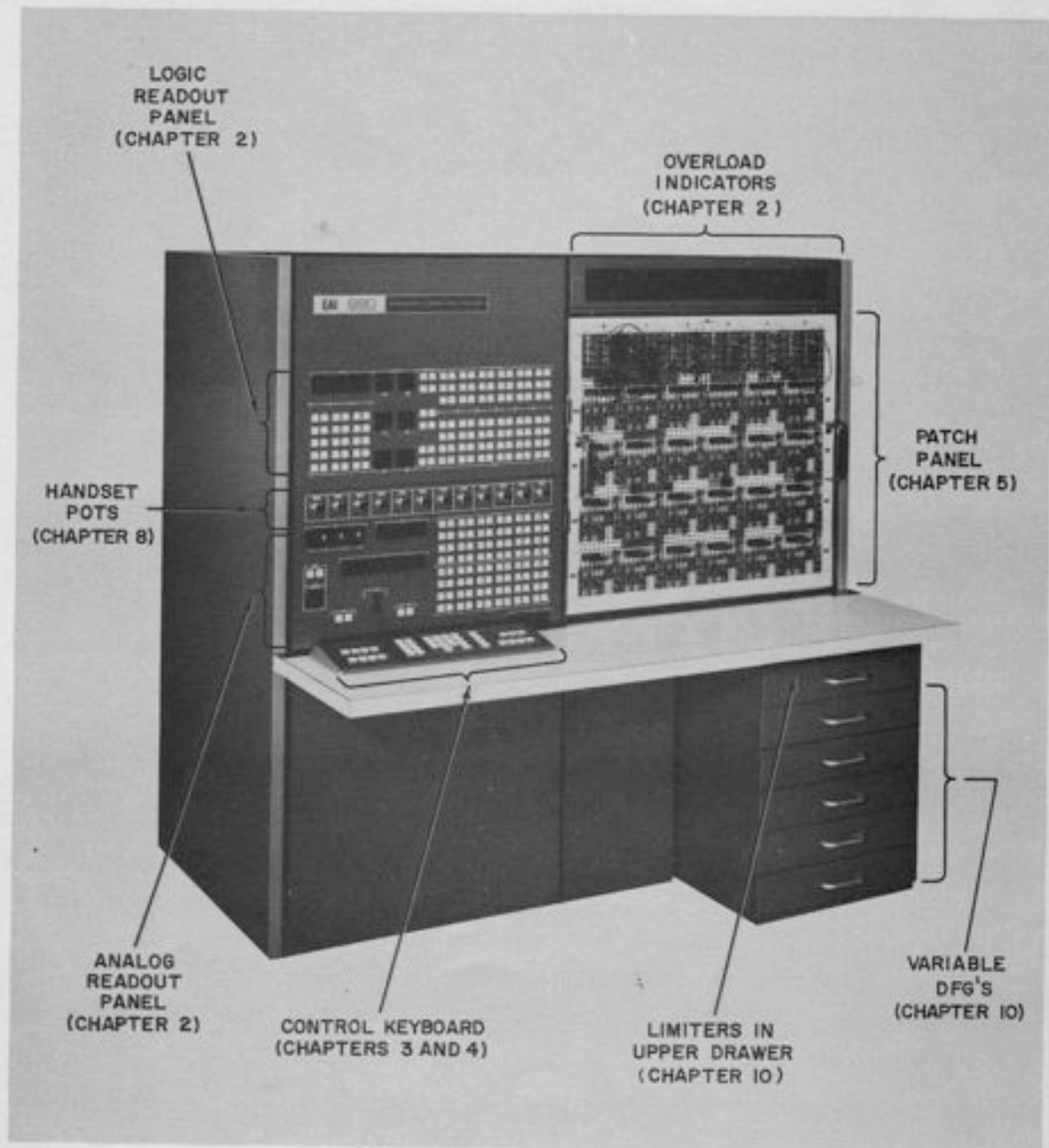
Figure 2.1. Overall View of the 680
