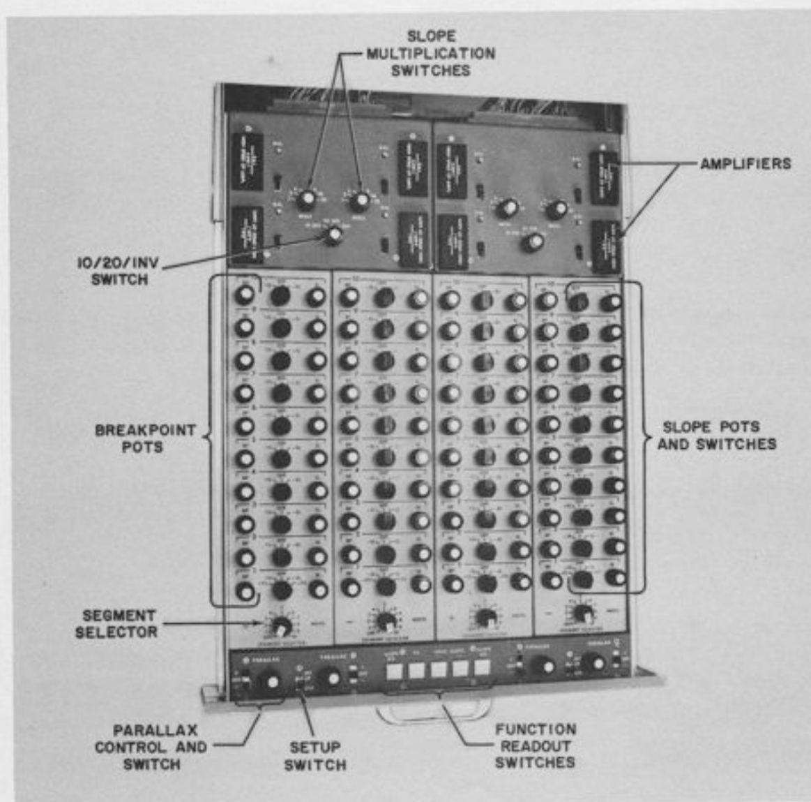
Figure 10.5. Typical DFG Drawer (Except for Upper Drawer)
