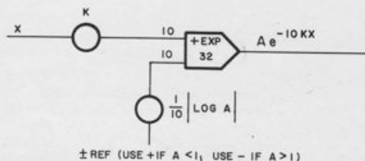
Figure A4.3. Exponential with Arbitrary Scale Factor
