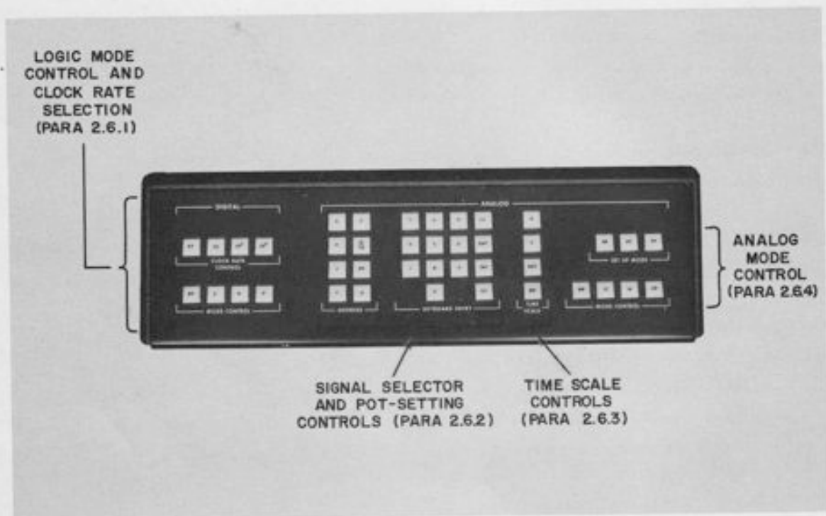
Figure 2.4. The Control Keyboard
