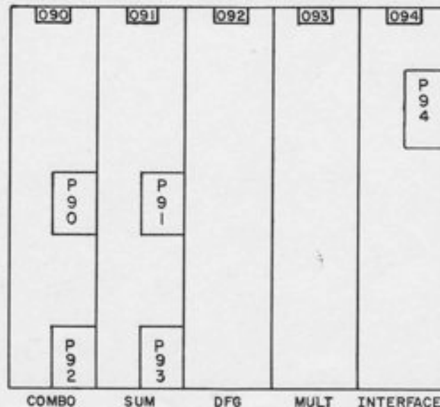
Figure 8.1. Servo-Set Pot Locations Within a Field
