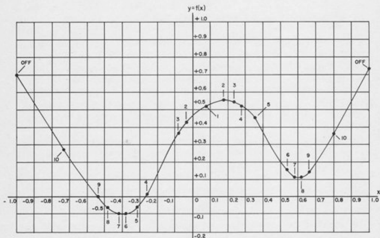
Figure 10.8. A Typical Twenty-Segment Function
