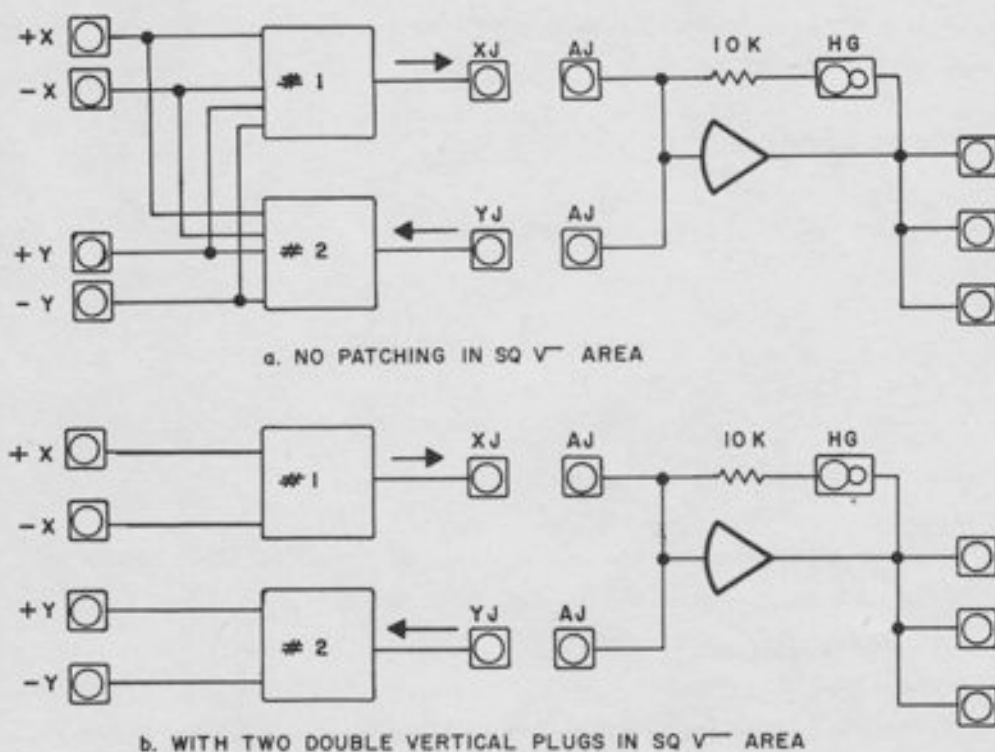
Figure 11.2. Quarter-Square Multiplier Equivalent Schematics
