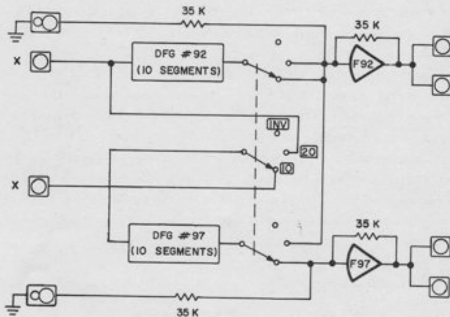
Figure 10.10. 10/20/INV Switching
