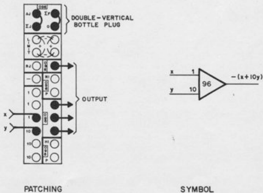
Figure A1.7. Summation with a Limit Summer
