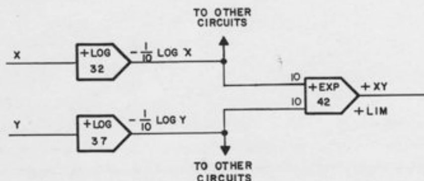
Figure A4.6. Multiplication - Many Products with Common Factors
