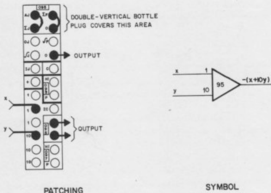
Figure A1.8. Summation with a Combination Amplifier
