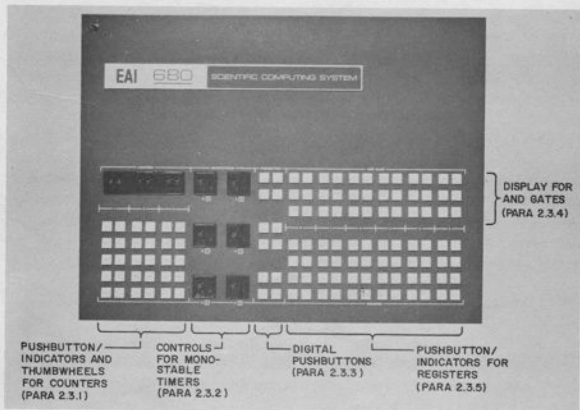
Figure 2.2. The Logic Readout Panel
