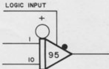
Figure A1.5. Abbreviated Symbol for the Integrator in Figure A1.4
