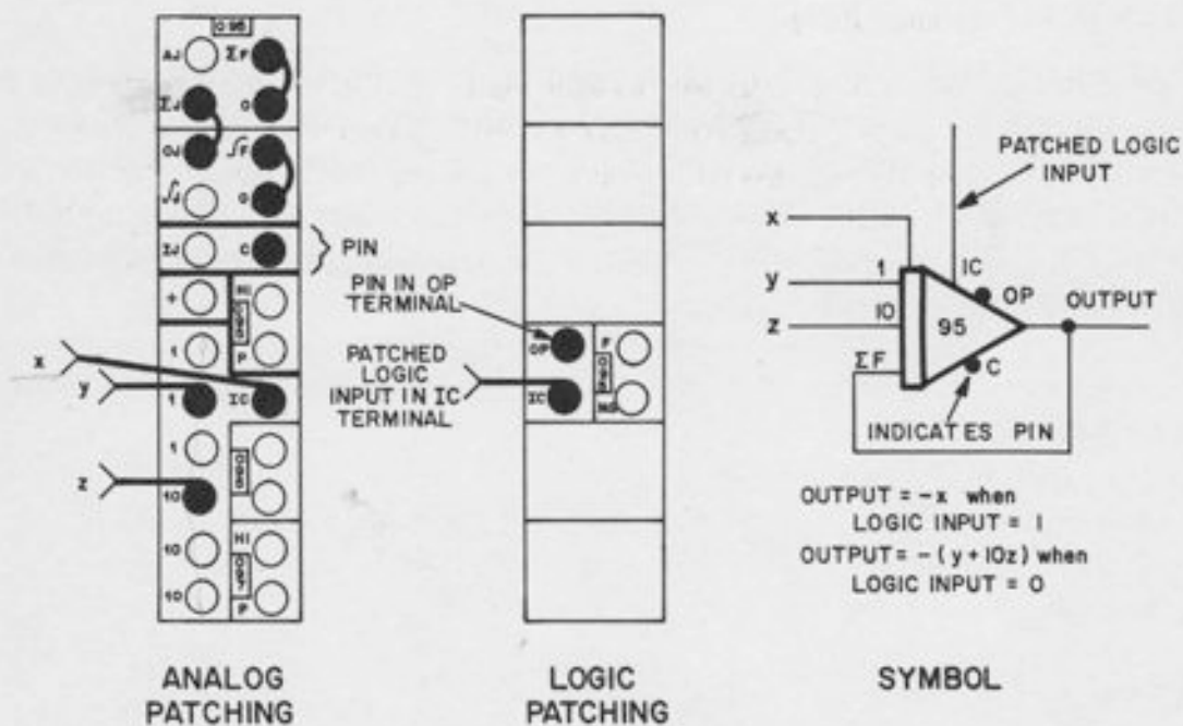
Figure A1.43. Use of the Combination Amplifier as an Electronic Switch
