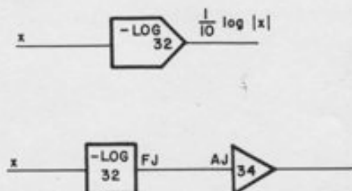
Figure A1.33. Logarithm, Using the -Log Network
