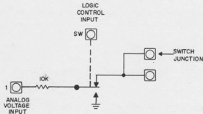
Figure 13.3. Relay Equivalent of D/A Electronic Switch
