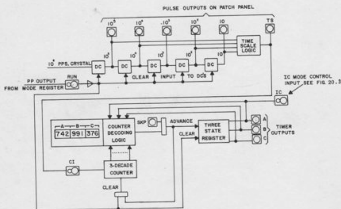
Figure 20.2. Timing Pulses and Rep-Op Timer
