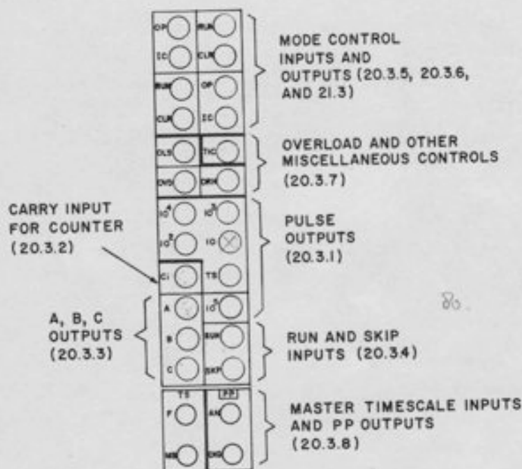
Figure 20.1. Mode Control/Timer Tray
