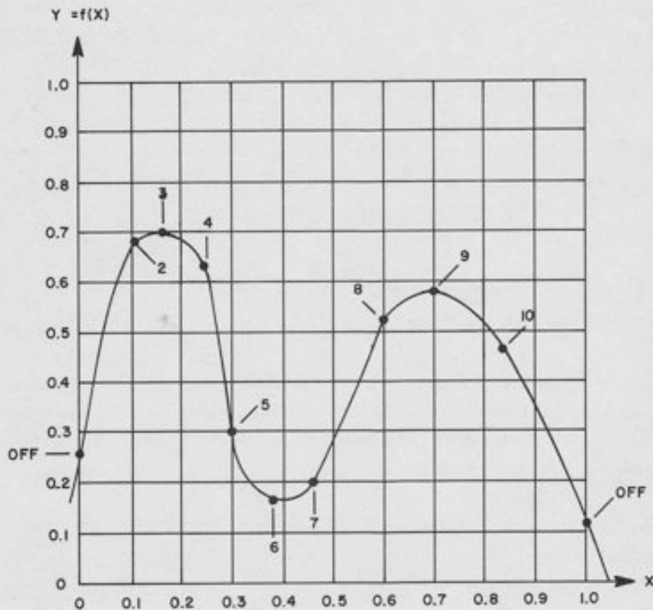
Figure 10.6. Typical Function Requiring Slope Amplification
