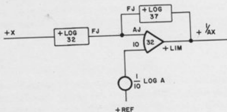
Figure A4.10. Reciprocal Generation
