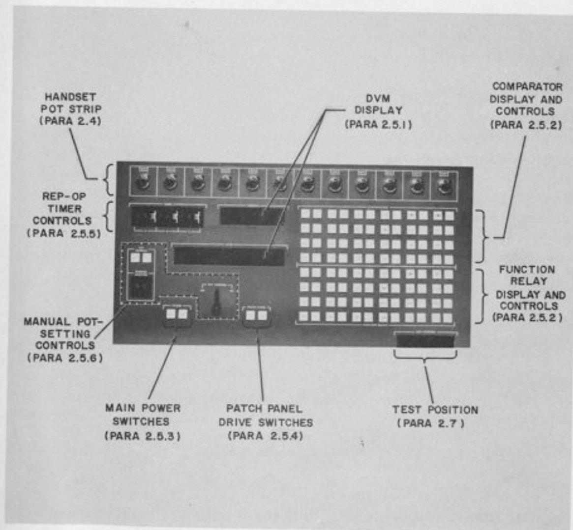
Figure 2.3. The Analog Readout Panel
