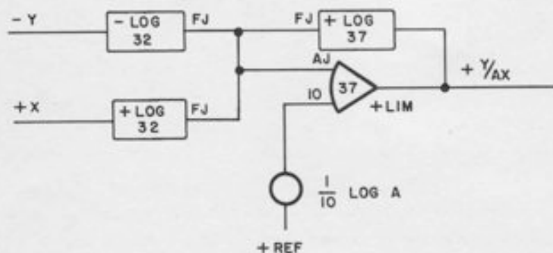
Figure A4.9. Division
