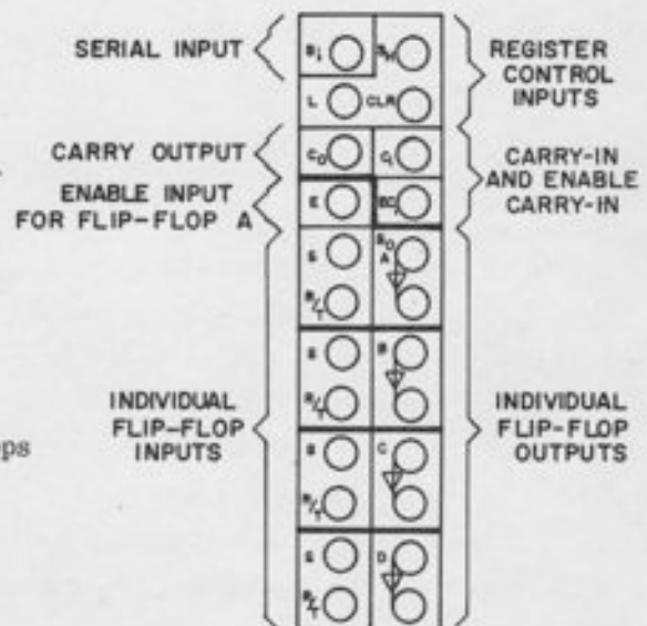
Figure 15.1. Patch Panel Terminations for a General-Purpose Register
