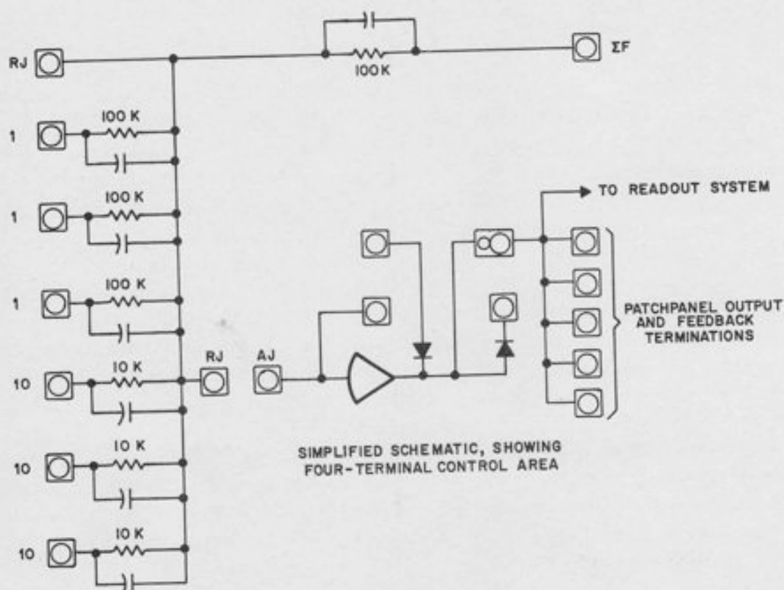
Figure 7.5. Simplified Schematic for Limit Summer
