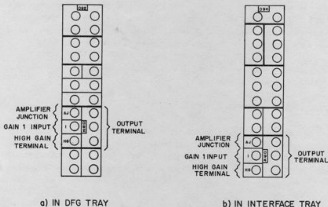
Figure 9.2. Junction Inverter Patching Areas
