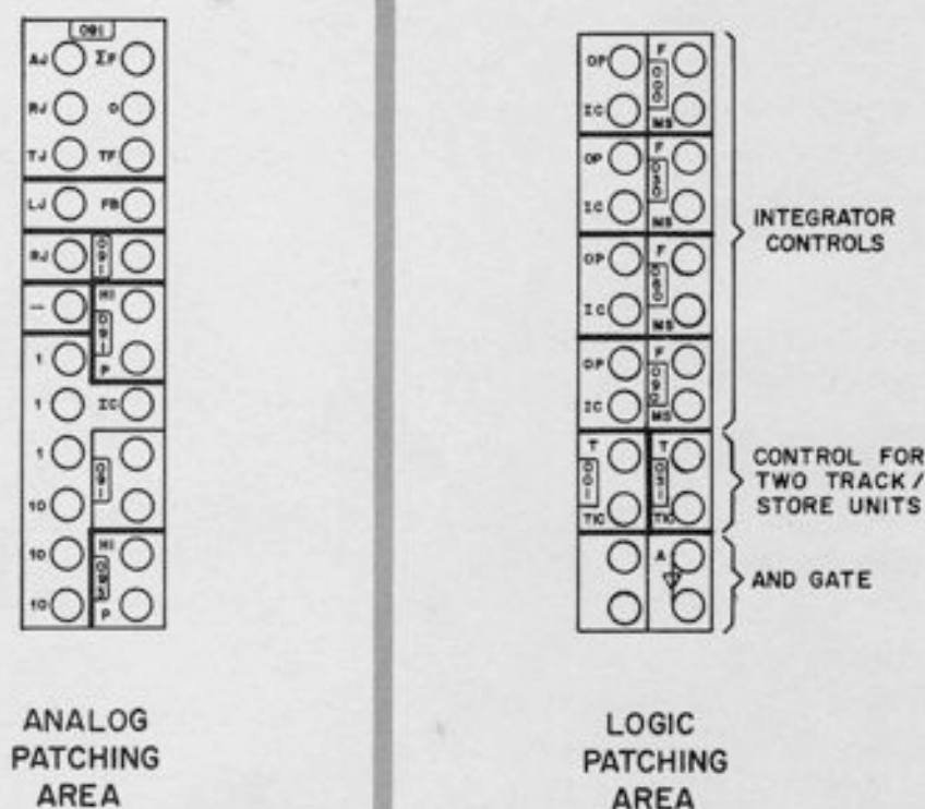
Figure 7.1. Patching Area for Track/Store Summer
