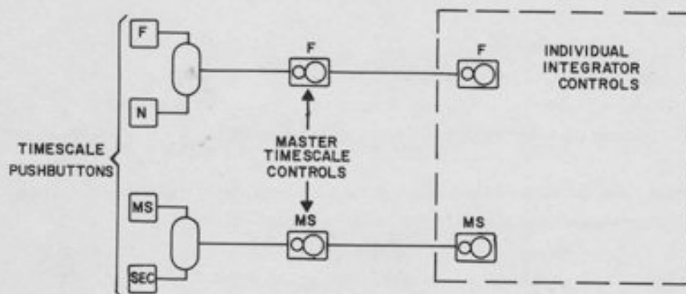
Figure 19.1. Master and Individual Time Scale Control
