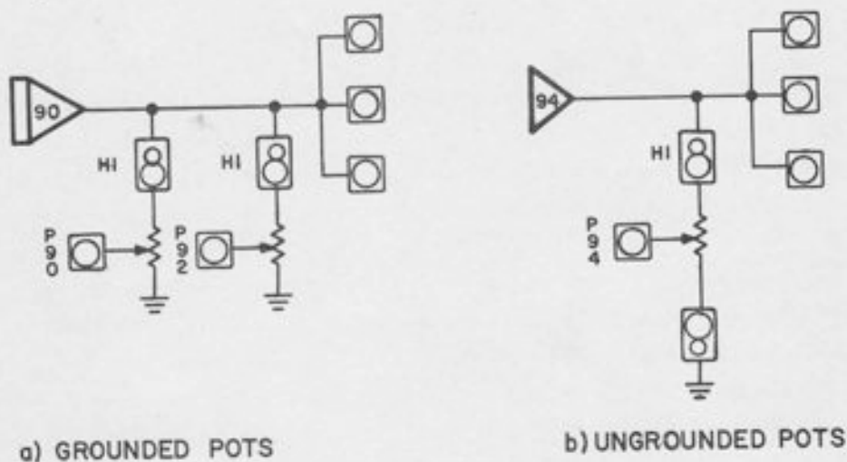
Figure 8.2. Normally-Closed Connections on Pots
