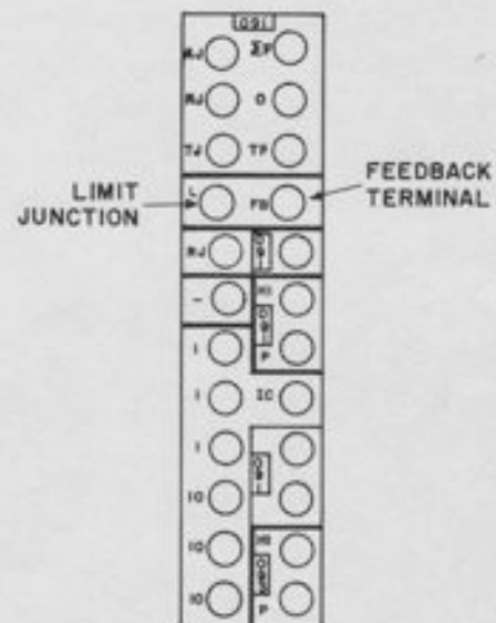
Figure 12.1. Patching Terminations for a Feedback Limiter
