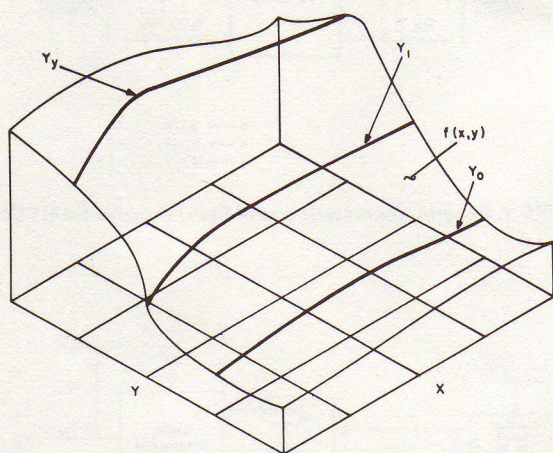
FIGURE 4. Function of Two Variables
