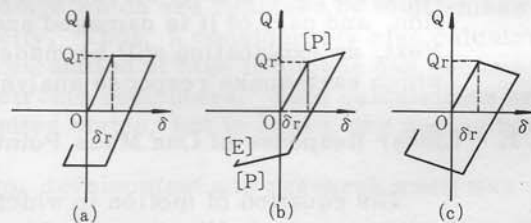
Fig. 13 Non-linear characteristics \delta \equiv Y = y - y_0
