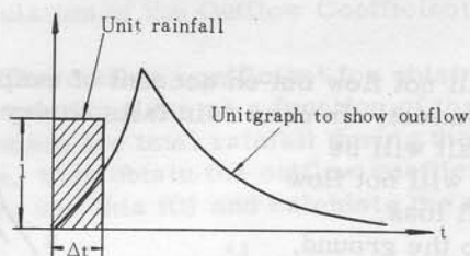
Fig. 5 Unit Graph
