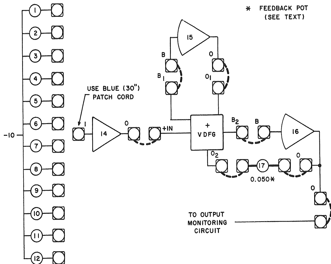
a. FUNCTION SETUP PATCHING (PREFERRED)
