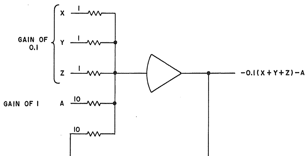
d. A HIGH-GAIN AMPLIFIER PATCHED FOR GAINS OF 0.1 AND 1
