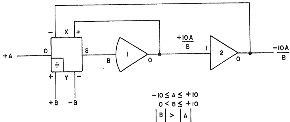
Figure 12. Division Circuit for a Quarter-Square Multiplier
