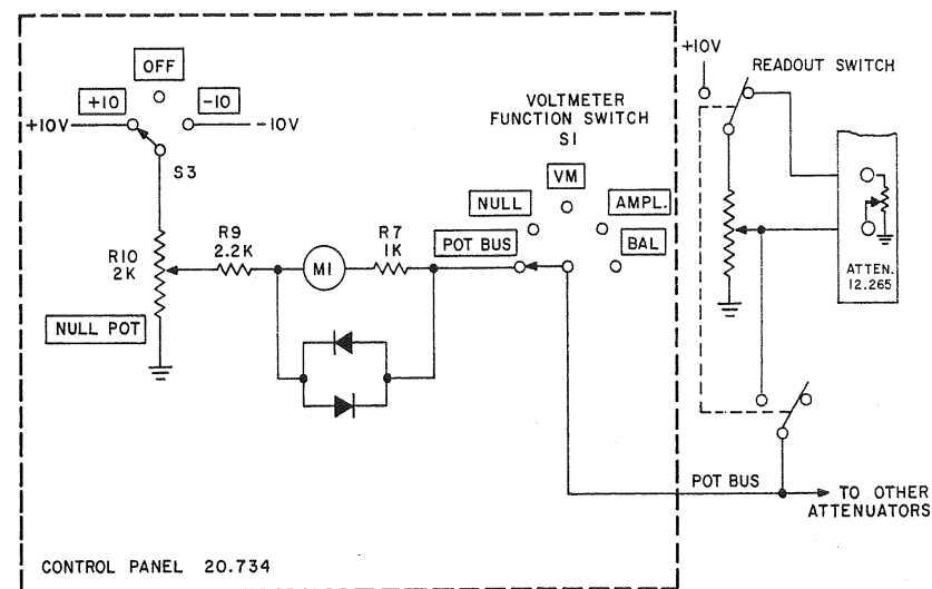
(e) POT BUS POSITION
