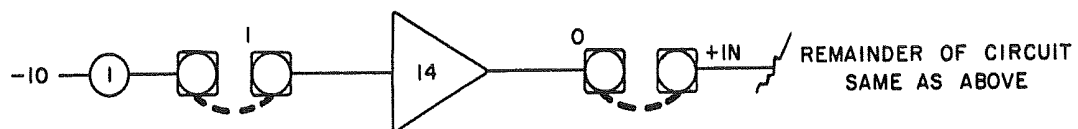
b. FUNCTION SETUP PATCHING (ALTERNATE METHOD)
