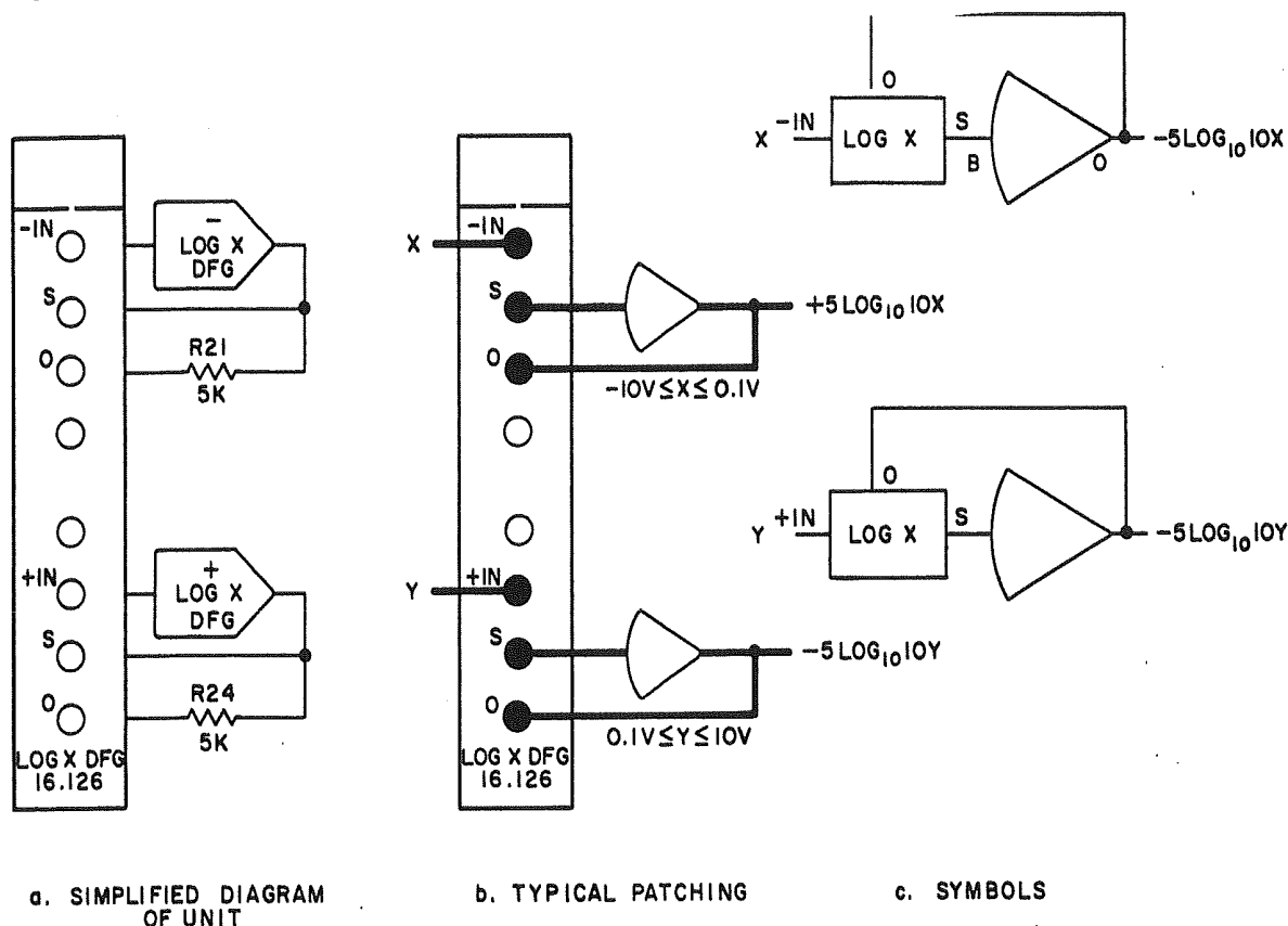
Figure 15. Patching the Log X DFG's
