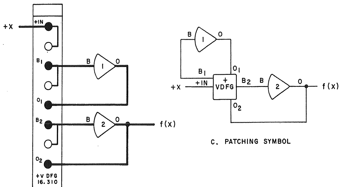
b. PATCHING
