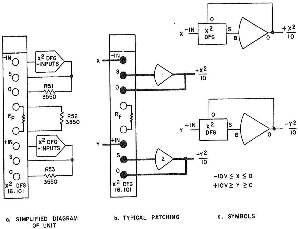
Figure 13. X^2 DFG Patching
