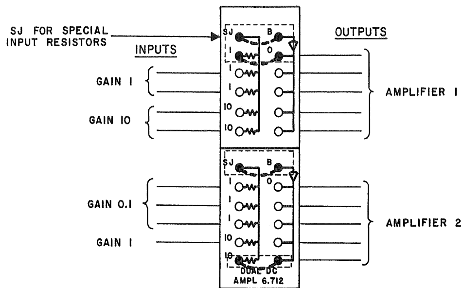
a. PATCHING WITH BOTTLE PLUGS
