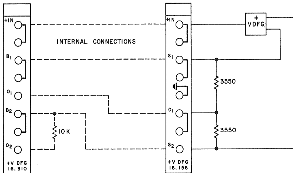
a. SIMPLIFIED SCHEMATIC
