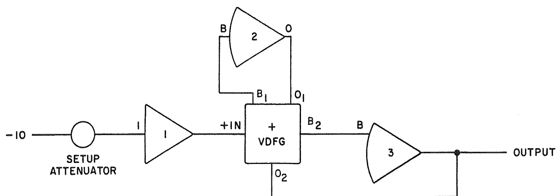
c. SETUP PATCHING
