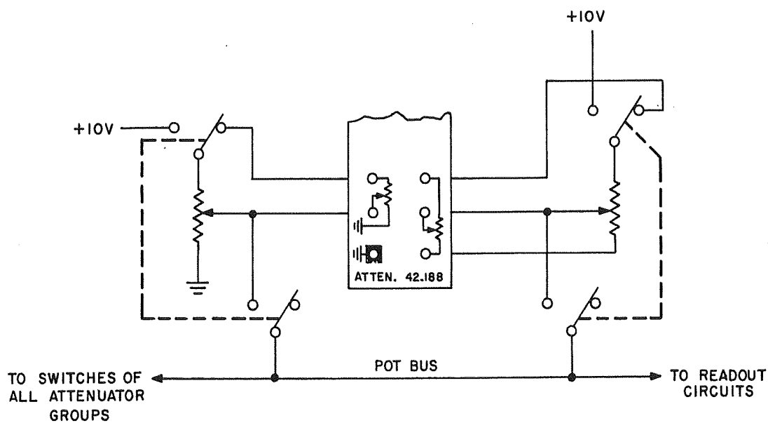
(a) ATTENUATORS, SIMPLIFIED SCHEMATIC
