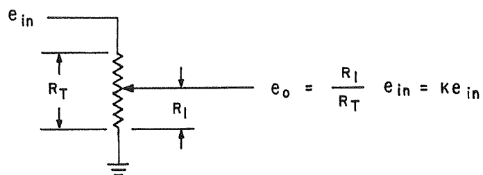
Figure 6. An Attenuator
